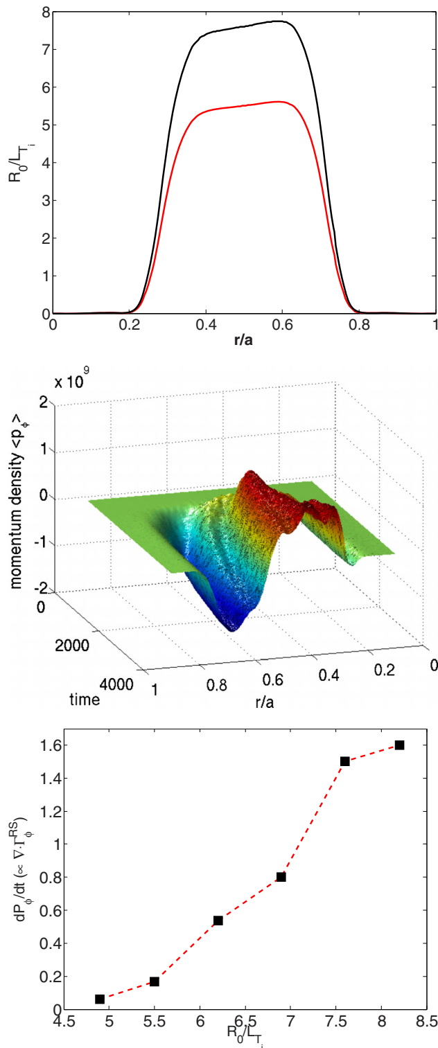
FIG. 8. (Color online) Radial profiles of R_0/L_{Ti} (illustrated are two cases with \kappa_{Ti}=5.5 and 7.6 ; top); spatiotemporal evolution of toroidal momentum density \langle p_\phi \rangle (flux-surface averaged; middle); and total intrinsic torque (spatially averaged) vs ion temperature gradient R_0/L_{Ti} (bottom).
