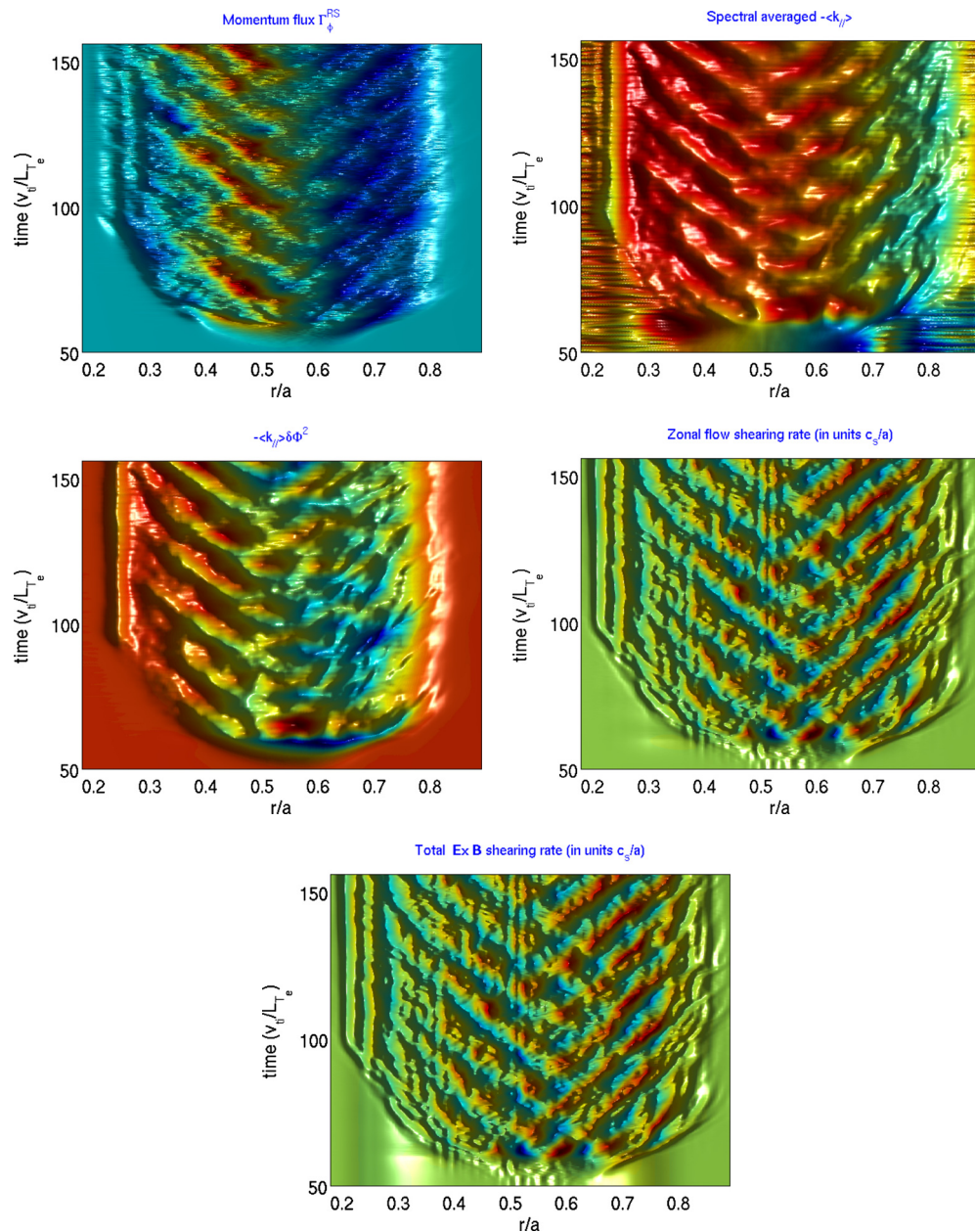
FIG. 13. (Color online) Spatiotemporal evolution of radial flux of toroidal momentum (top-left), \langle k_\parallel \rangle \Sigma \delta \Phi_{mn}^2 (midleft), spectrum-averaged \langle k_\parallel \rangle (top-right), zonal flow shearing rate (midright), and total \mathbf{E} \times \mathbf{B} shearing rate (bottom) from simulation of CTEM turbulence.
