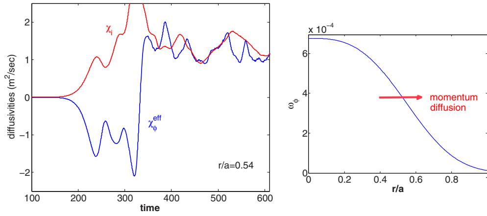
FIG. 4. (Color online) Time evolution of effective toroidal momentum and heat diffusivity (left) and initial toroidal rotation profile (right). Time unit is L_{Ti}/v_{th} .
