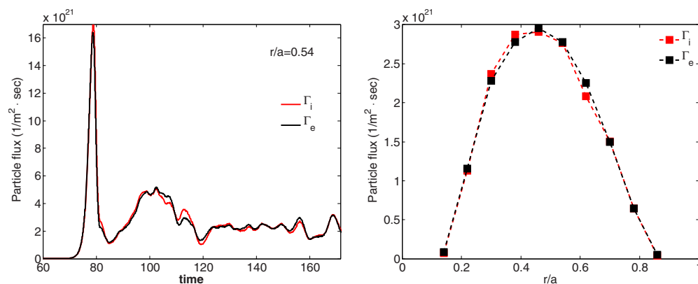
FIG. 2. (Color online) Time history of ion and electron particle fluxes (left) and steady state ion and electron particle fluxes vs minor radius r (right). Time unit is L_\eta/c_s . This is from the same simulation as that in Fig. 1.
