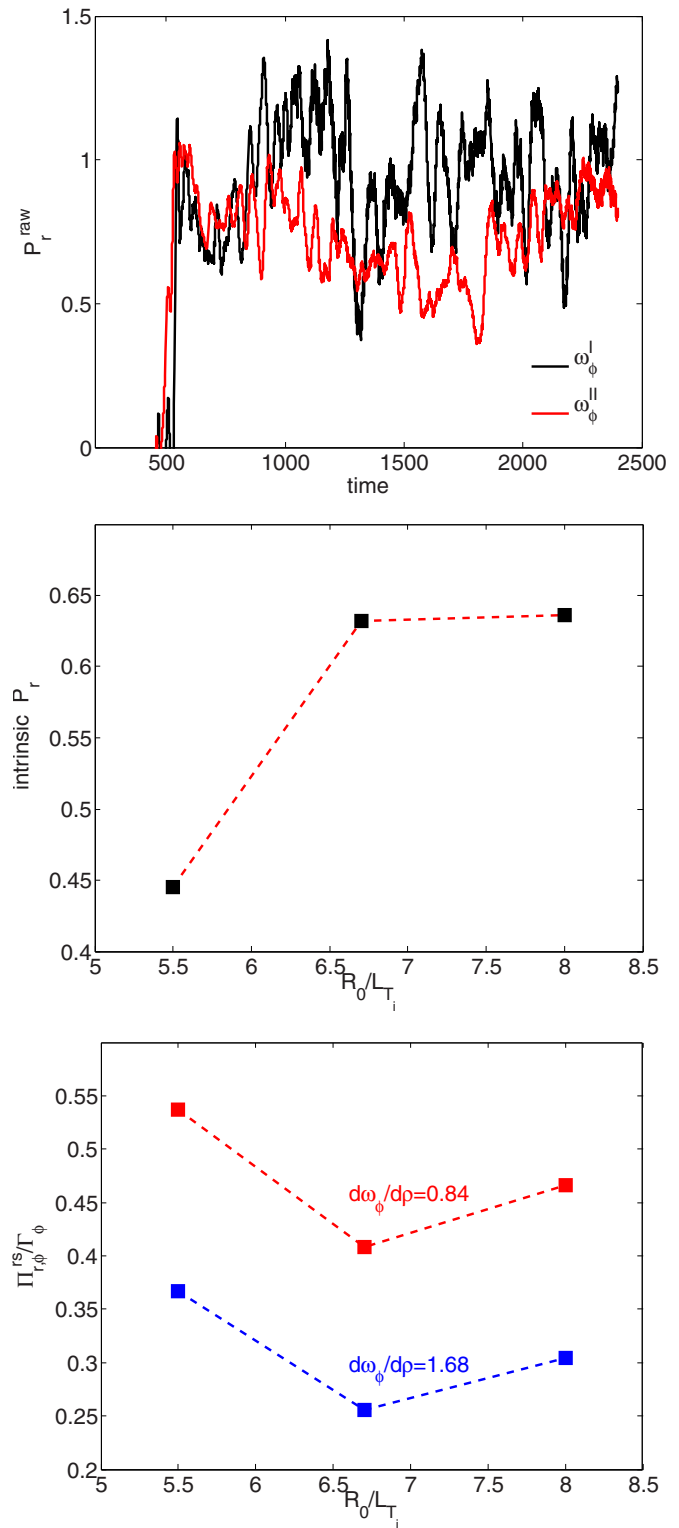
FIG. 6. (Color online) Time (normalized by L_T/v_{th} ) evolution of raw Prandtl number from two simulation with R_0/L_{Ti}=5.5 and different rotation gradients (top), intrinsic Prandtl number vs R_0/L_{Ti} (middle), and ratio of residual stress over total momentum flux vs rotation gradient and R_0/L_{Ti} (bottom).
