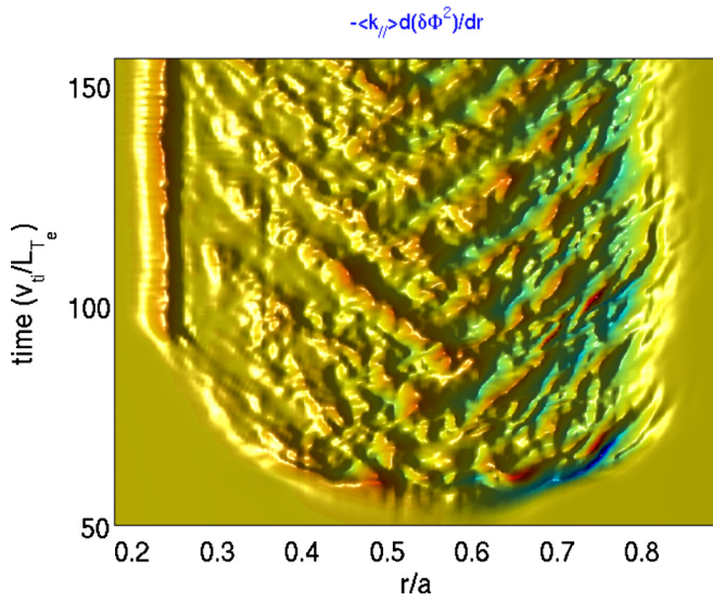
FIG. 14. (Color online) Spatiotemporal evolution of \langle k_{||} \rangle \Sigma \partial / \partial r (\delta \Phi^2) , which represents the part of the residual stress driven by the turbulence intensity gradient.
